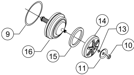
#1 CHECK ASSEMBLY (350 & 450 2 1/2" & 3")
